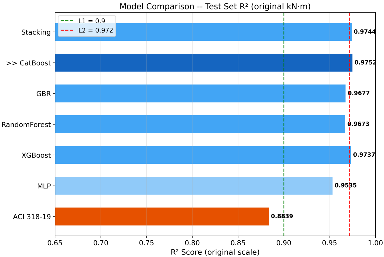
Fig6 Model Comparison
