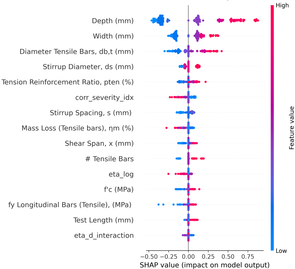
SHAP Beeswarm Plot — Feature Impact on R(%) Prediction
