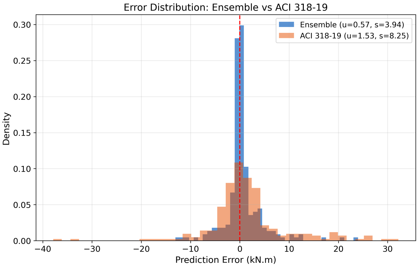
Fig6 Model Comparison
