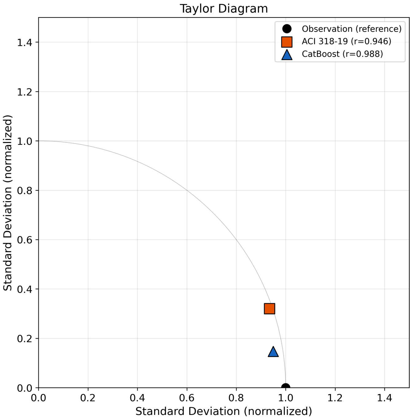
Fig7 Taylor Diagram
