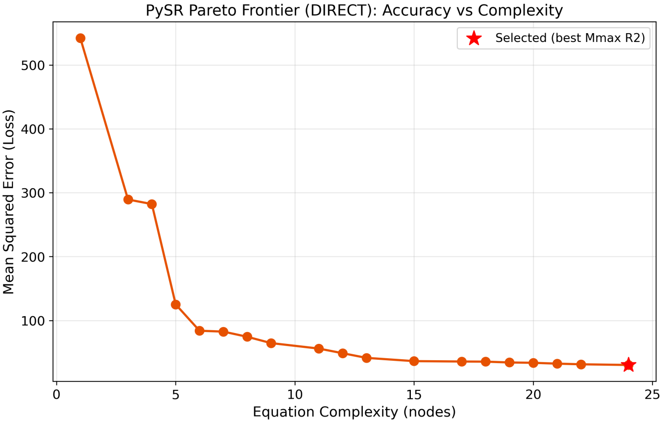
Fig9 Pareto Curve
